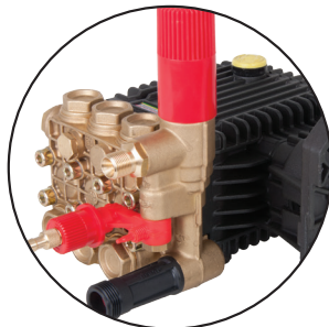
Interpump 63 Series
